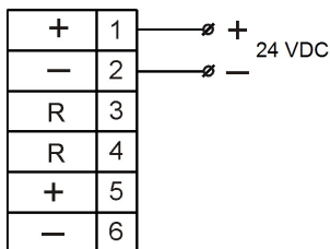
а) BC-07e-Ex-3(И)-24VDC
