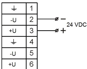
б) BC-07e-Ex-СД-24VDC
