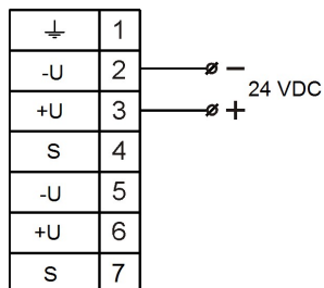
в) BC-07e-Ex-СЛ-24VDC
