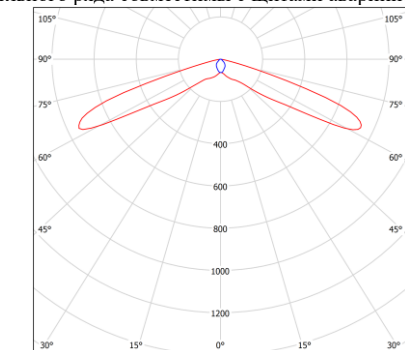
L2 C0 - C180 C90 - C270
