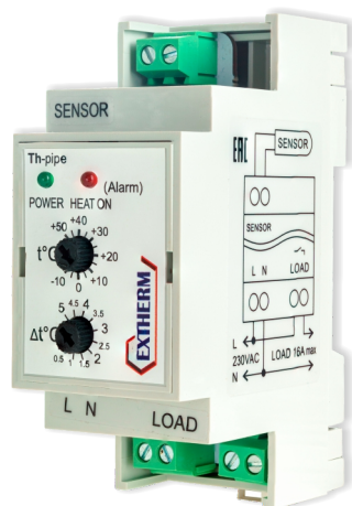
Extherm Th-pipe
