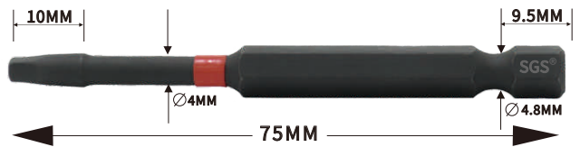
6.35mm系列单头方形冲击批头(S2材料) 1/4" Hexagon driver series Square impact screw bits(S2 material)
