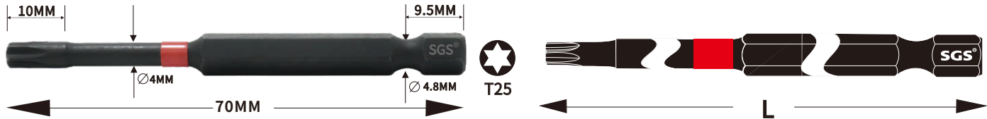
■ 6.35mm系列梅花不带孔冲击批头(S2材料) 1/4" Hexagon driver series Torx impact screw bits(S2 material)
