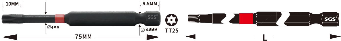
■ 6.35mm系列梅花带孔冲击批头(S2材料) 1/4" Hexagon driver series tamper proof Torx impact screw bits(S2 material)
