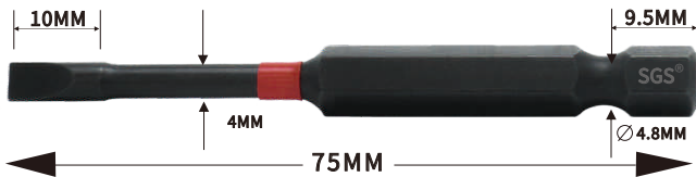
6.35mm系列单头一字冲击批头(S2材料) 1/4" Hexagon driver series Slotted impact screw bits(S2 material)
