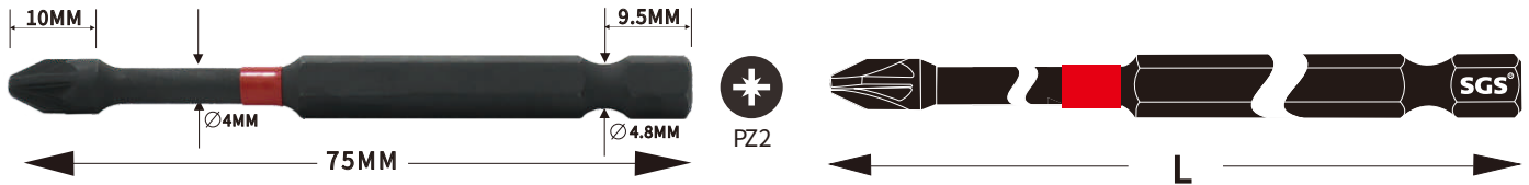
6.35mm系列单头米字冲击批头(S2材料) 1/4" Hexagon driver series Pozidriv impact screw bits(S2 material)
