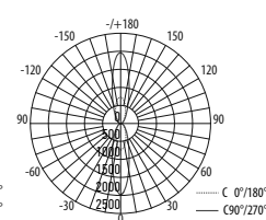
PWL-245110/24D 2x12W IP65
