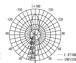
PWL-26090/24D 2x5W IP65
