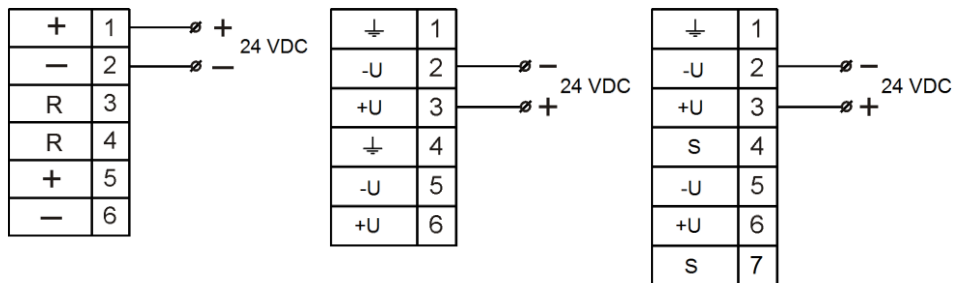
а) BC-07e-O-3(И)-24VDC
