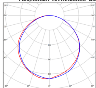
L1 cd/km C0 - C180 C90 - C270
