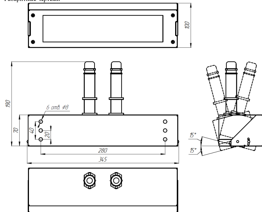
Рис.2 - BS-DBU-53-L2-INEXI3-AUTOTEST
