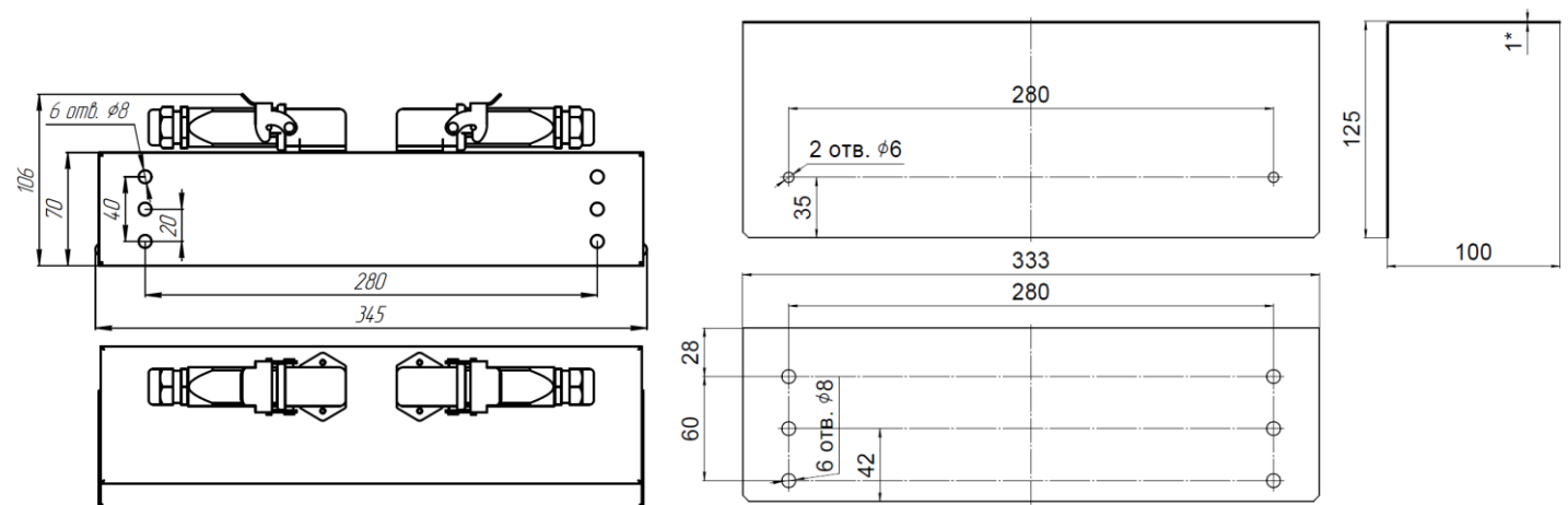
Рис.3 - BS-DBU-53-L2-INEXI3-AUTOTEST
