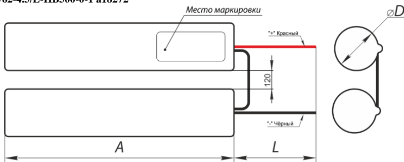
Рис.8 Батарея BS-3+3KRHT23/43-1.5/L-HB500-0-1 a18268 Батарея BS-3+3KRHT33/62-4.5/L-HB500-0-1 a18272
