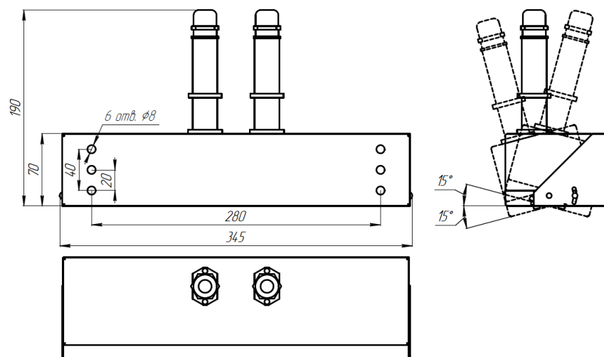
Рис.2 - BS-DBU-53-L1-INEX12
