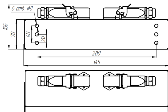
Рис.3 - BS-DBU-53-L2-INEX12
