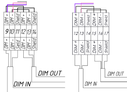
FORWARD 450 DMX
