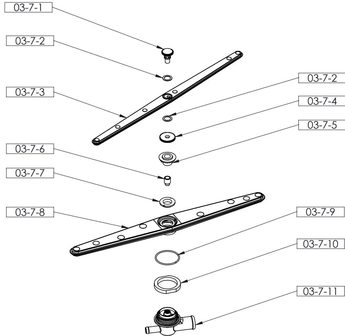
DETAIL OF / DETAY 03-7
