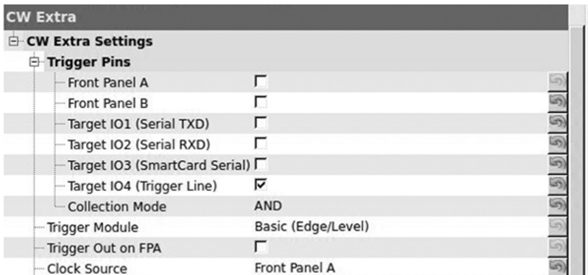
Figure 8-24: Glitch setup in the CW Extra Settings
