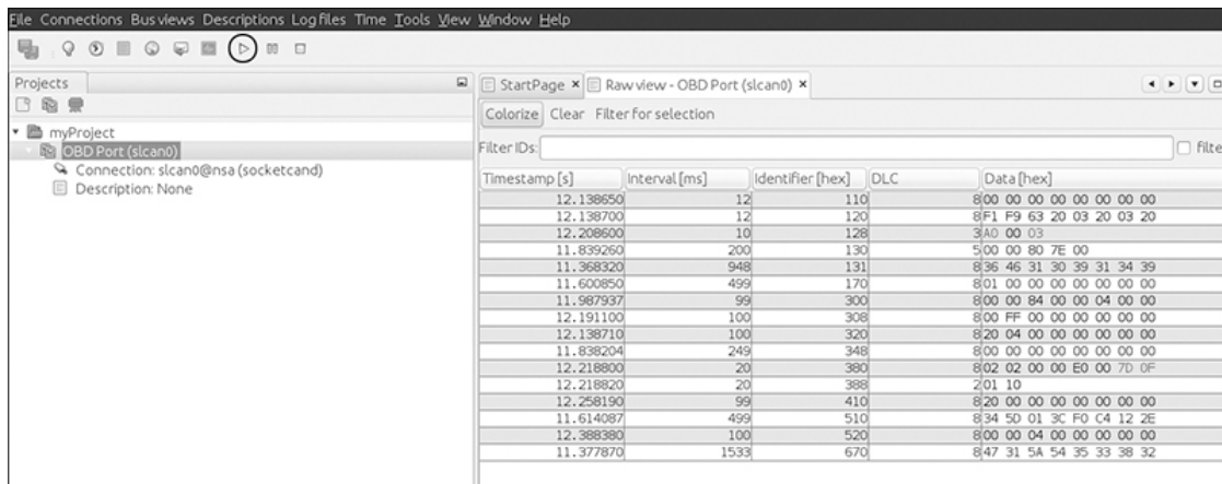
Figure 3-6: Open RAW view and press the play button to see packets from the CAN bus.
