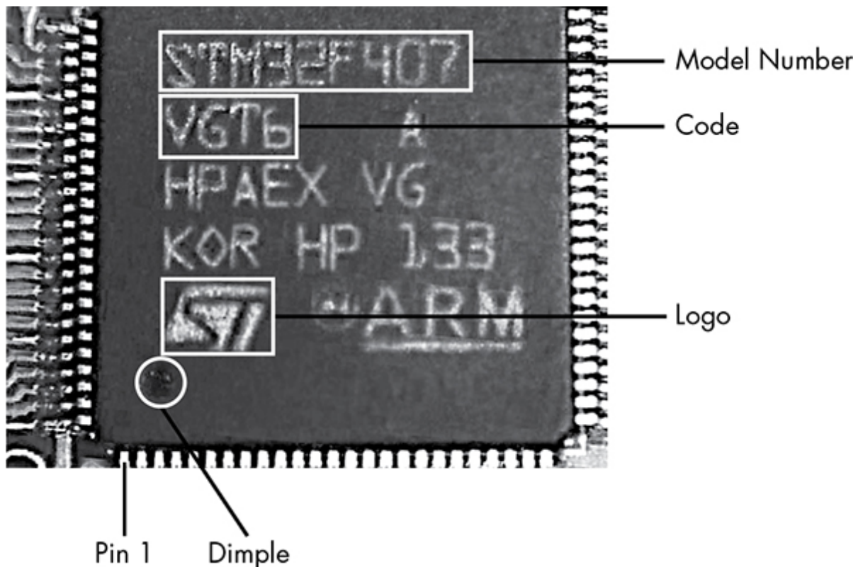
Figure 8-1: STM32 chipset identification
