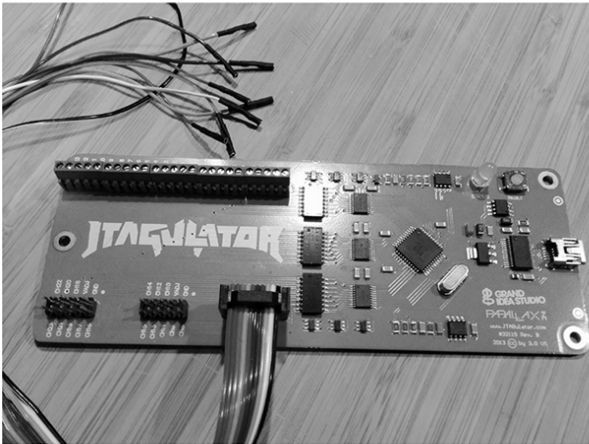
Figure 8-3: JTAGulator with a Bus Pirate cable
