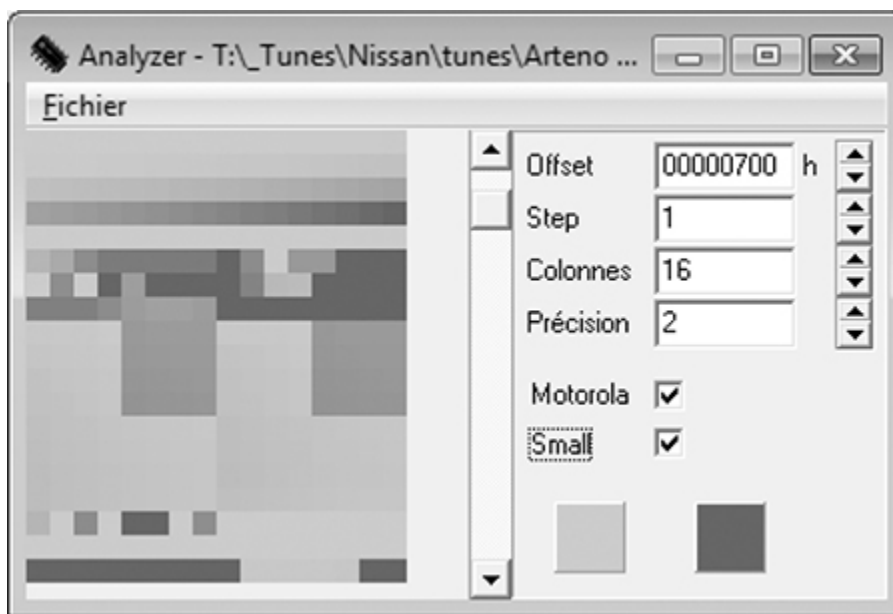
Figure 6-5: First four rows of 16×16-bit values
