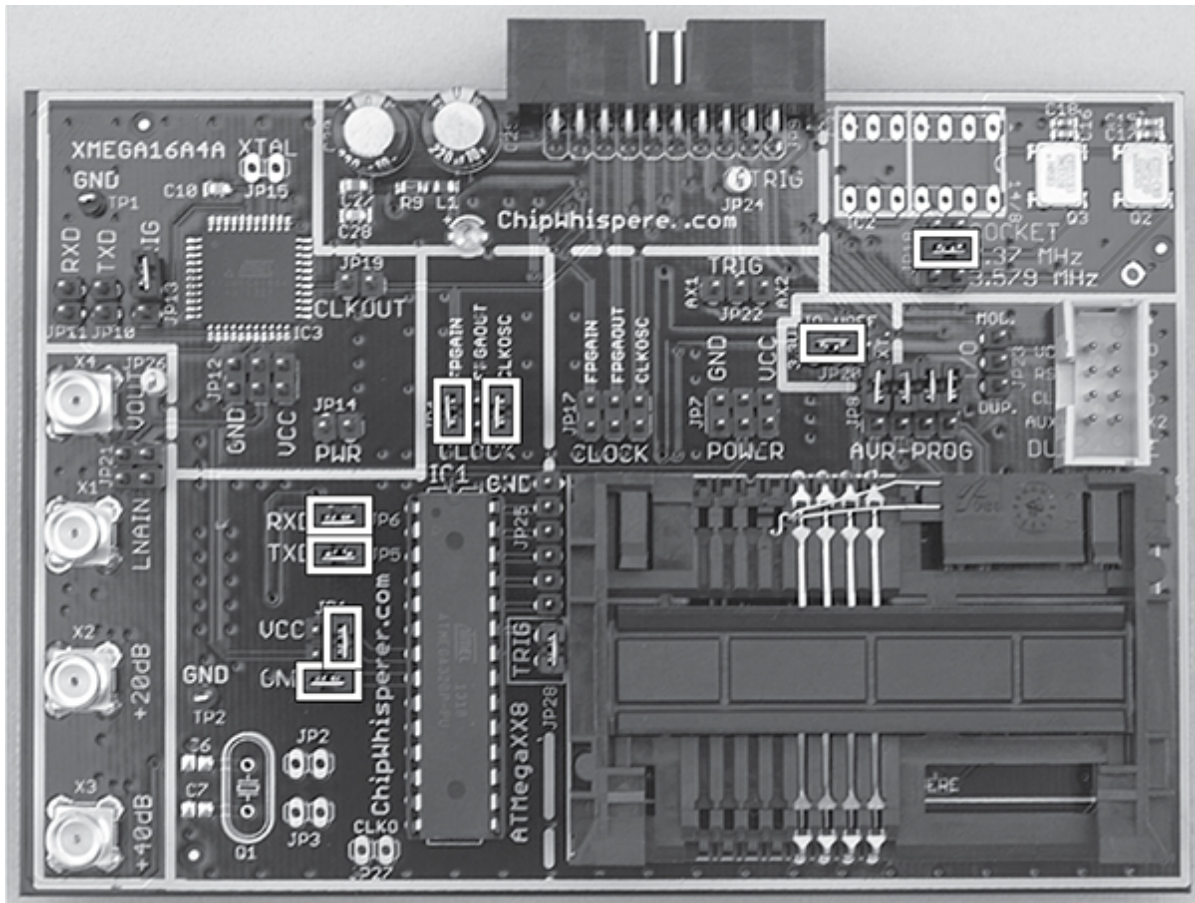
Figure 8-7: Jumper settings for the MultiTarget Victim Board
