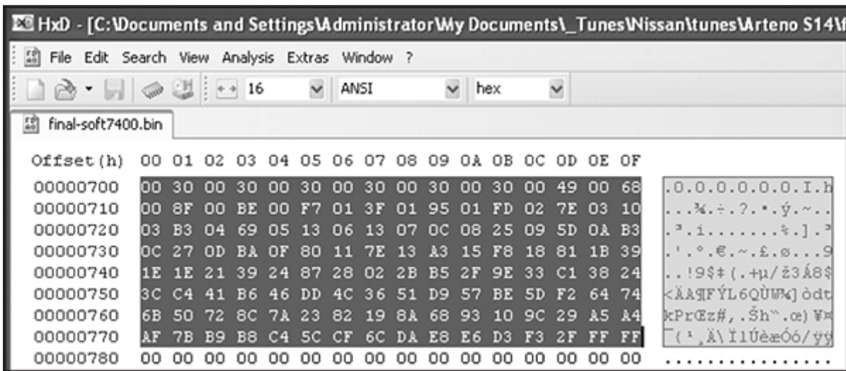
Figure 6-3: VQ table in HxD hex editor: 128 bytes or 64- to 16-bit words
