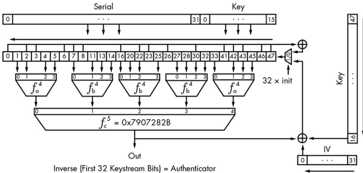
Figure 12-7: Hitag 2 cipher
