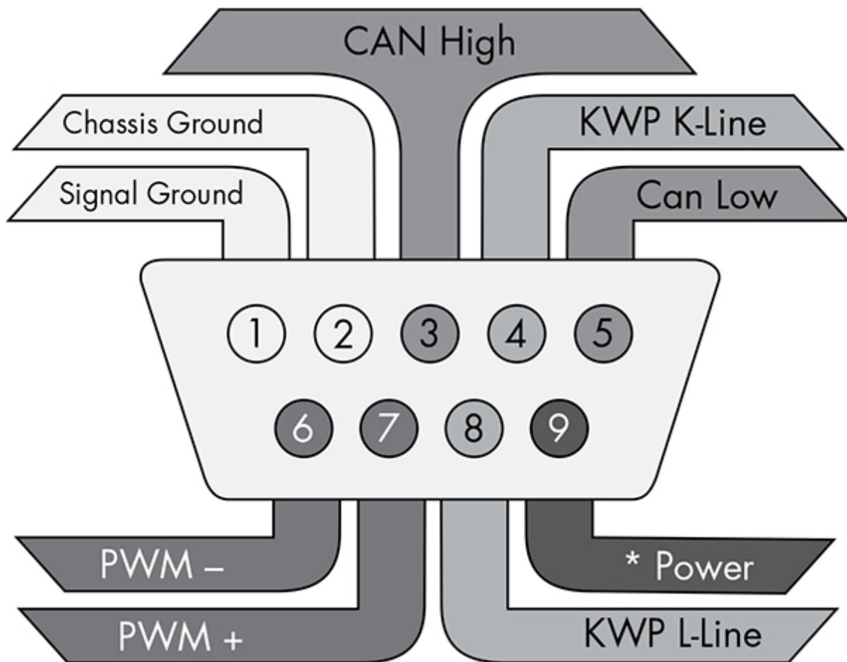
Figure 2-19: US-style DB9 connector, plug view
