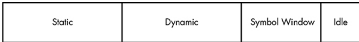
Figure 2-13: Four parts of a FlexRay cycle
