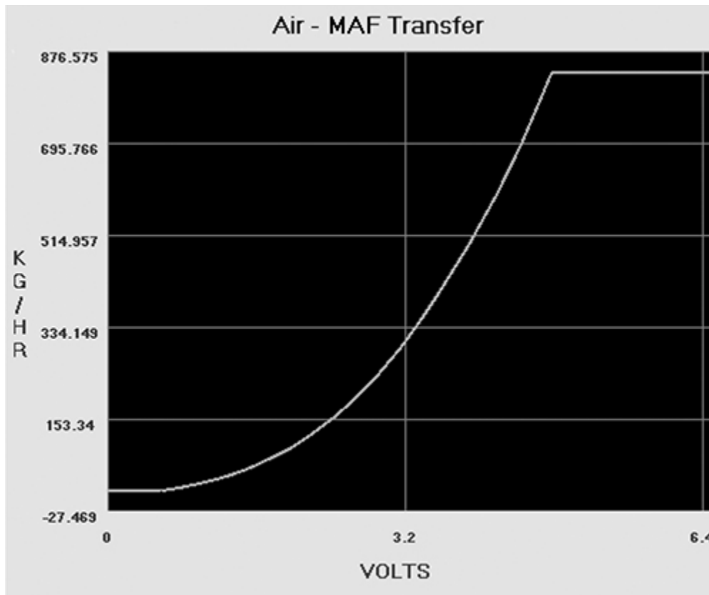
Figure 6-1: Ford MAF transfer graph
