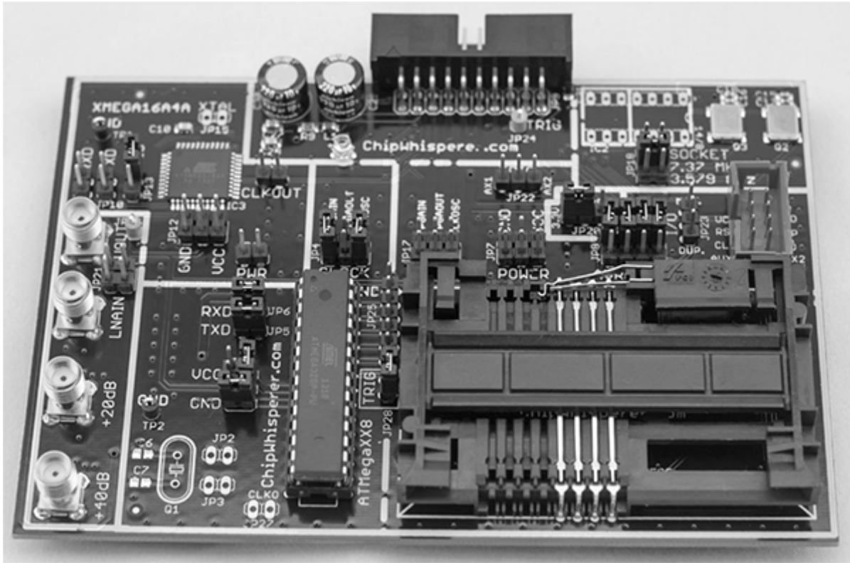
Figure 8-6: MultiTarget Victim Board
