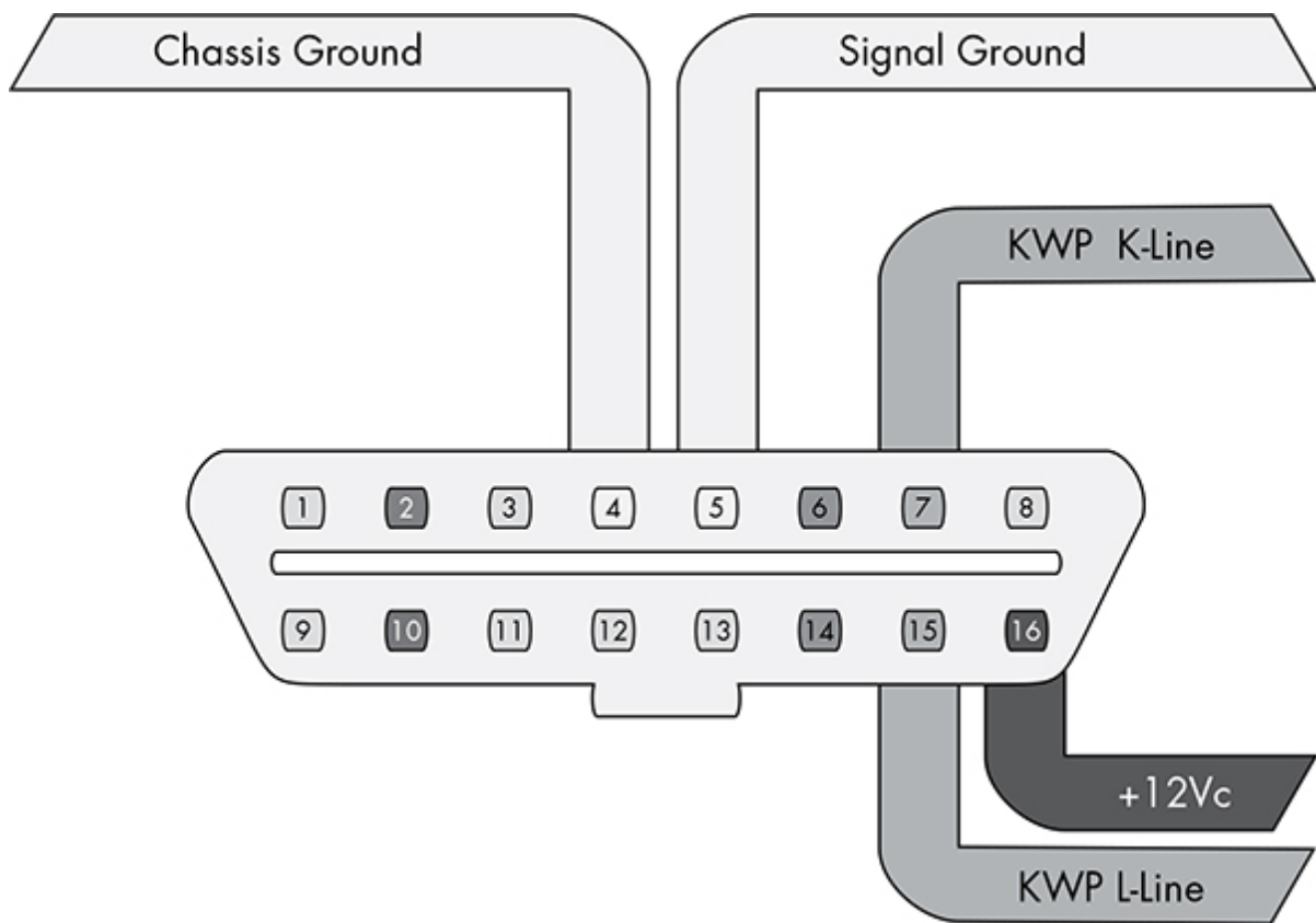
Figure 2-7: KWP K-Line pins cable view
