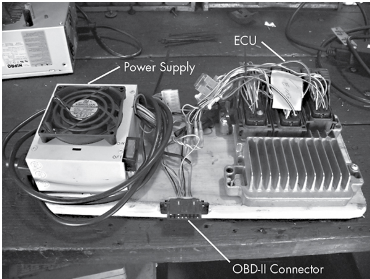
Figure 7-1: A simple ECU test bench
