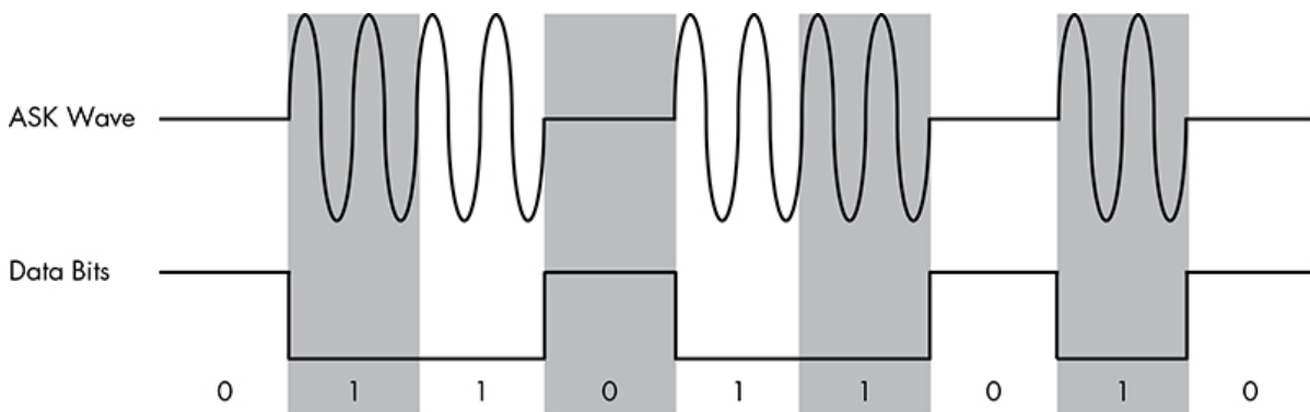
Figure 12-1: ASK modulation
