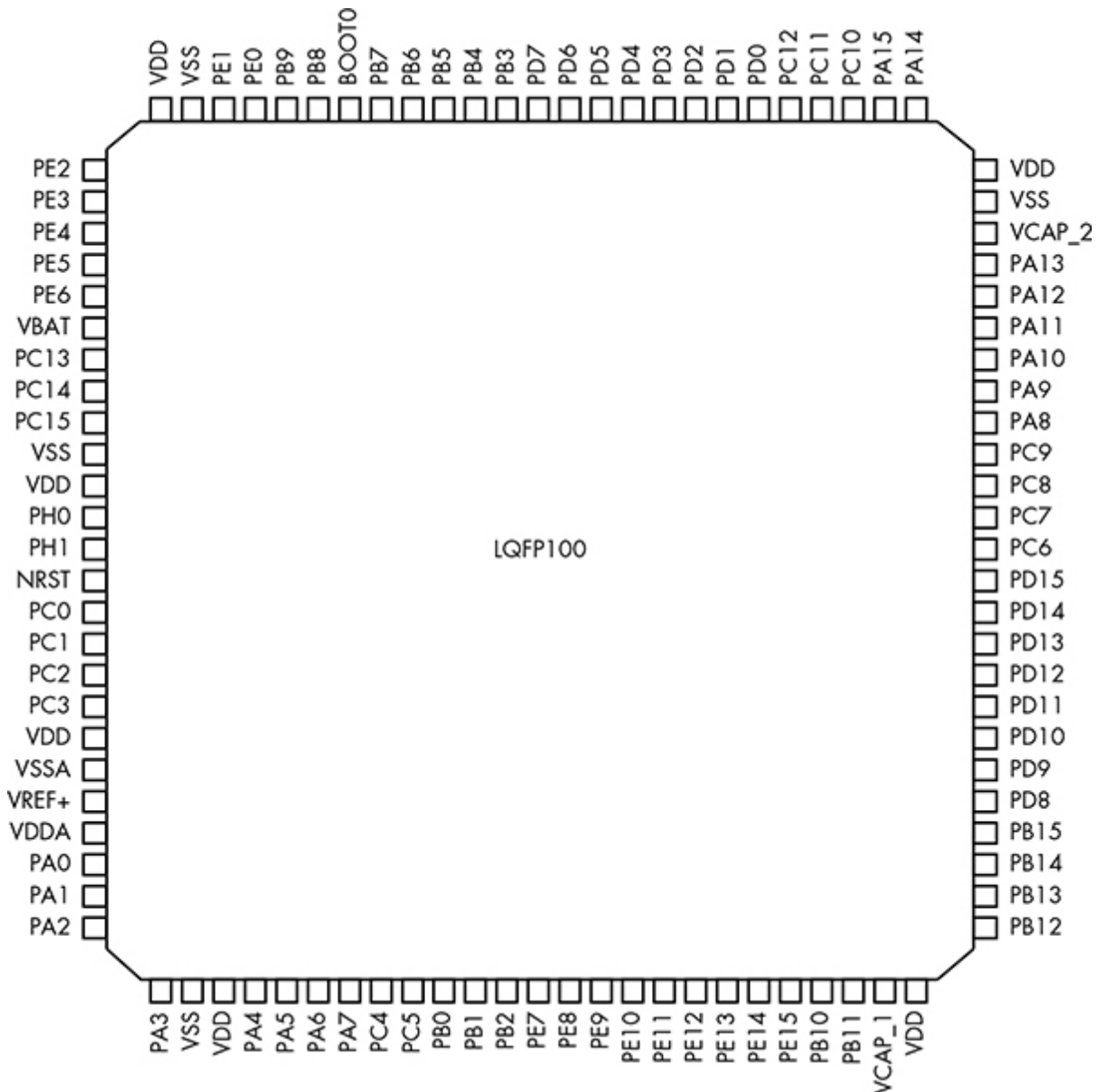
Figure 8-2: STM32F4 data sheet pinout
