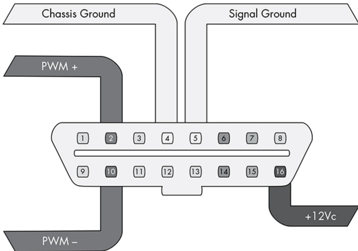
Figure 2-5: PWM pins cable view
