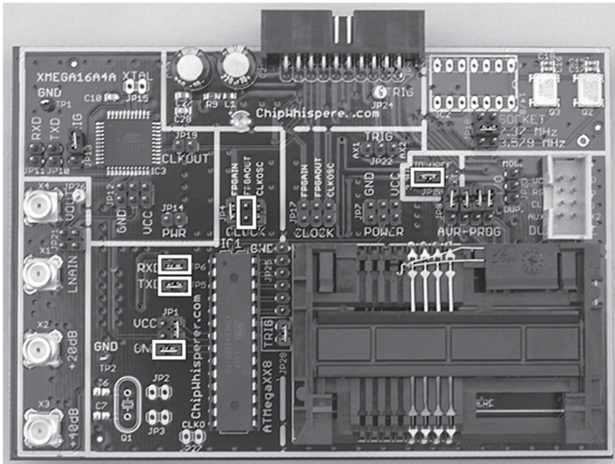
Figure 8-20: MultiTarget Victim Board set for glitching
