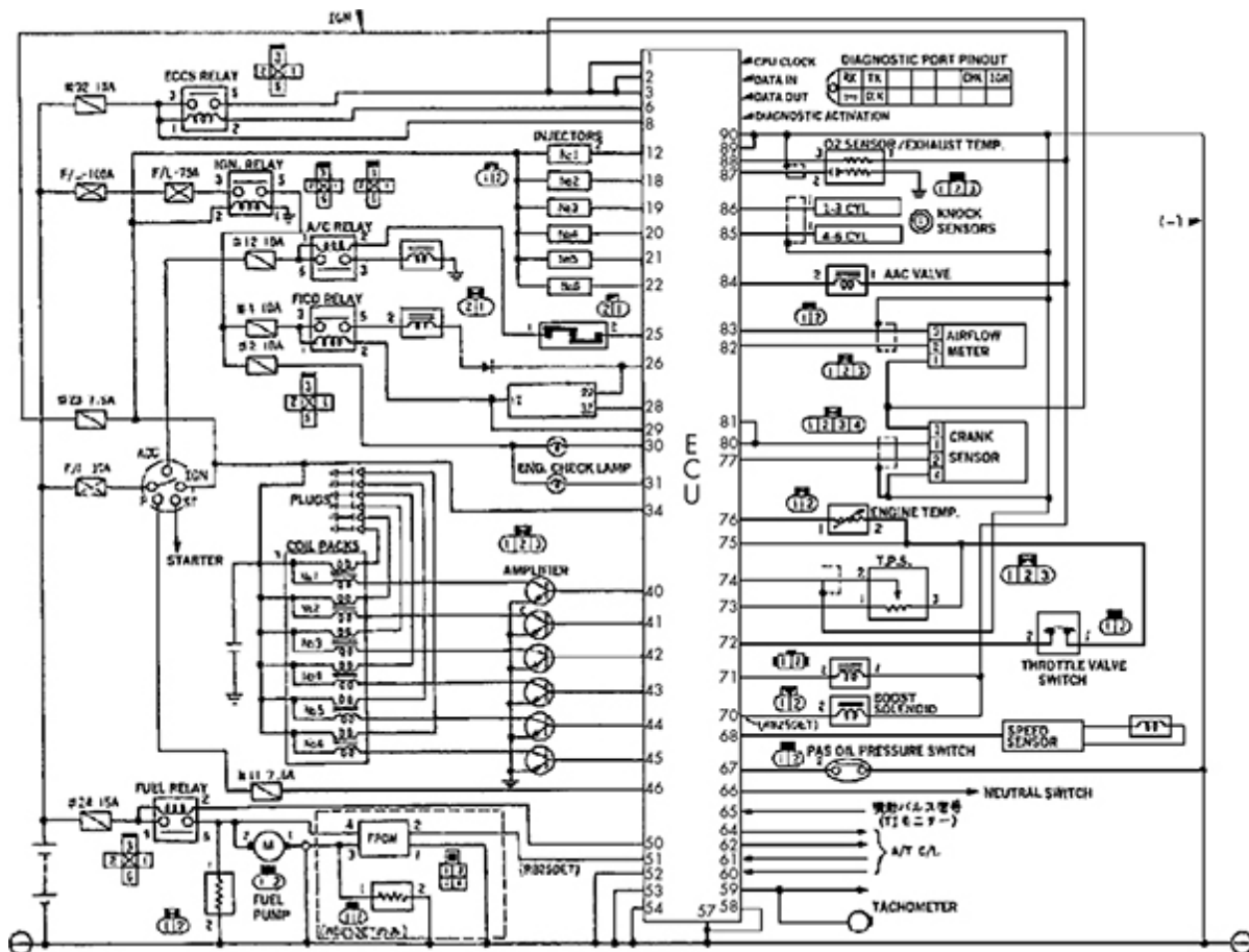
Figure 7-3: Example of an ECU wiring diagram
