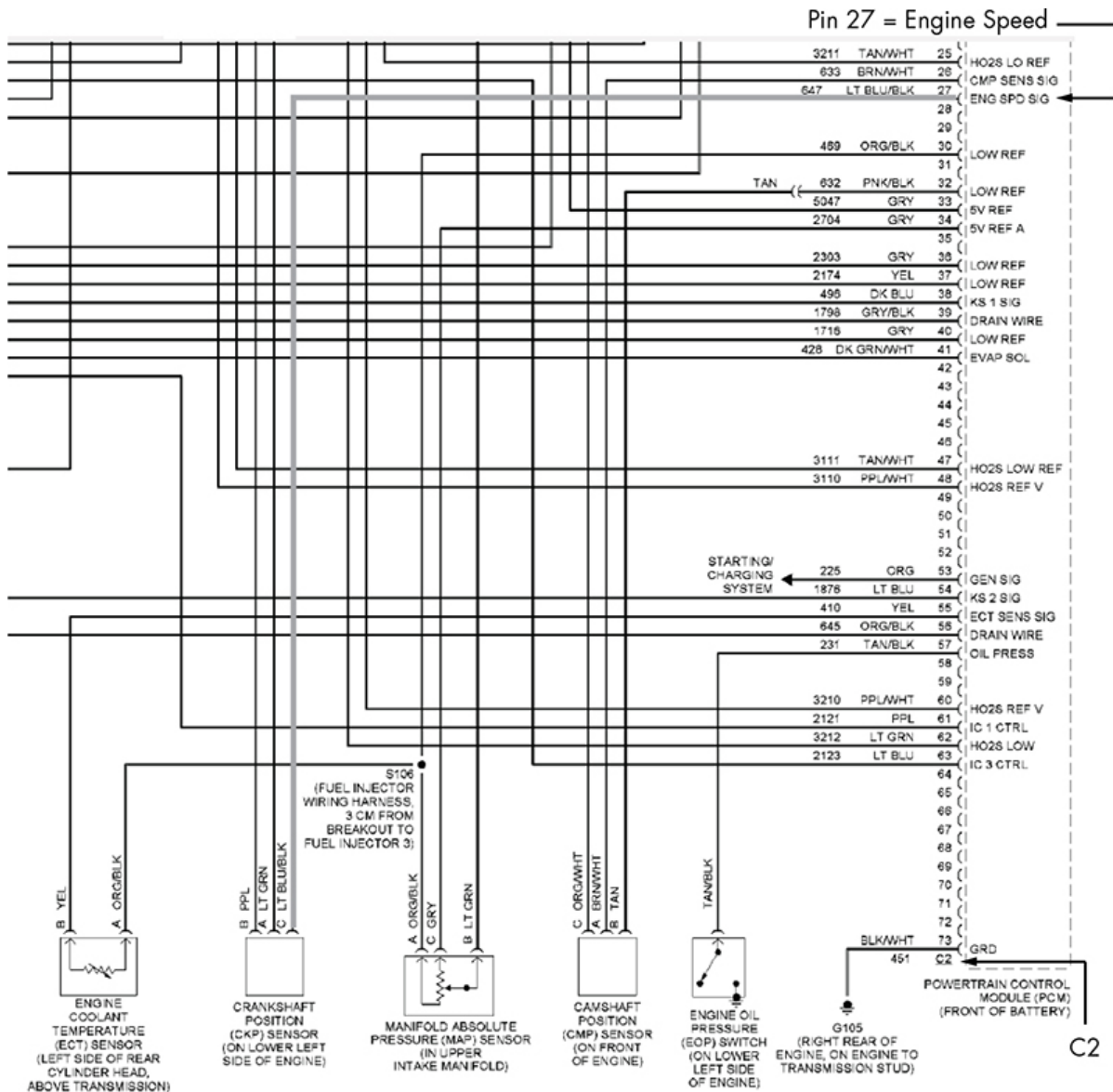
Figure 7-8: Wiring diagram showing the engine speed pin
