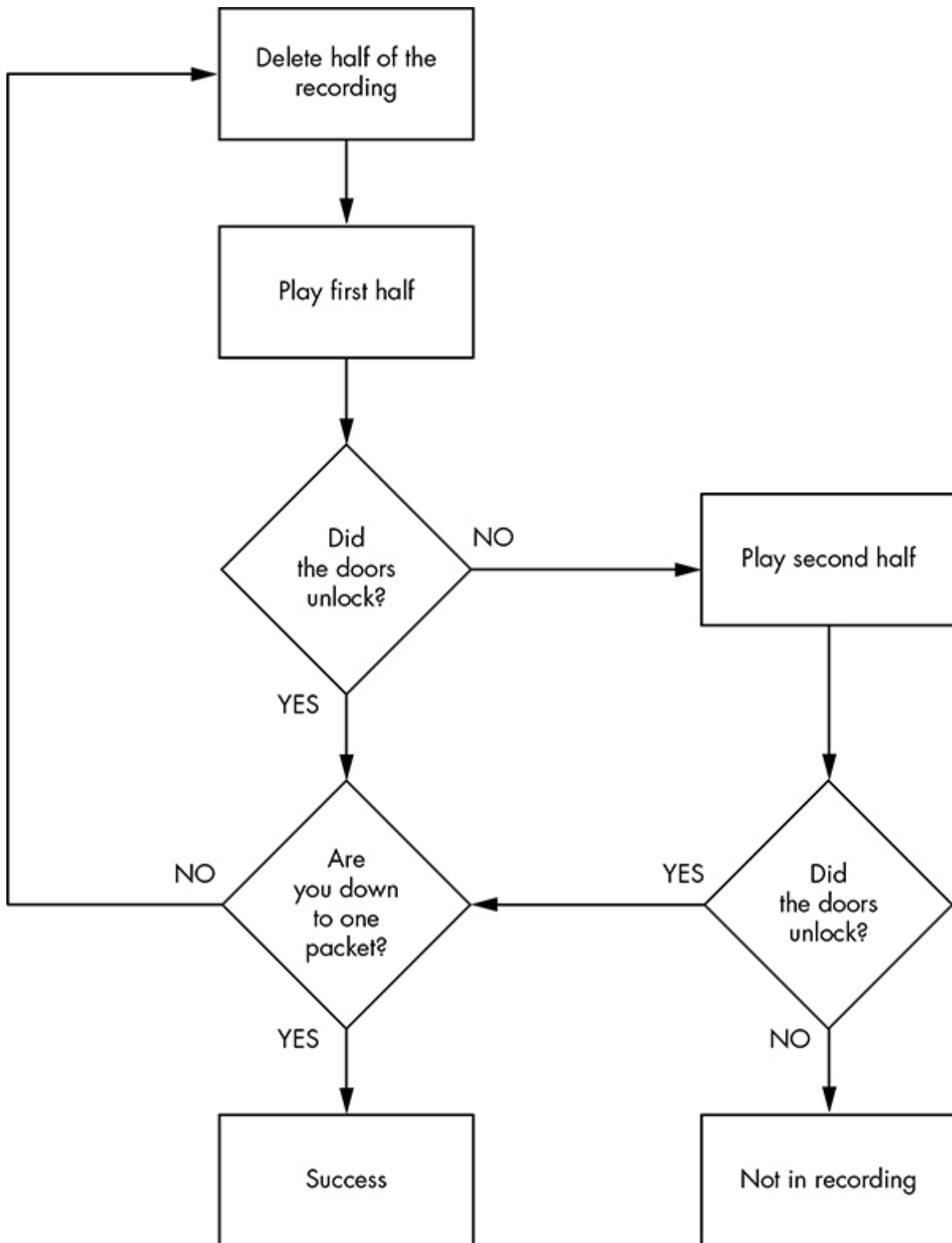
Figure 5-6: Sample unlock reversing flow
