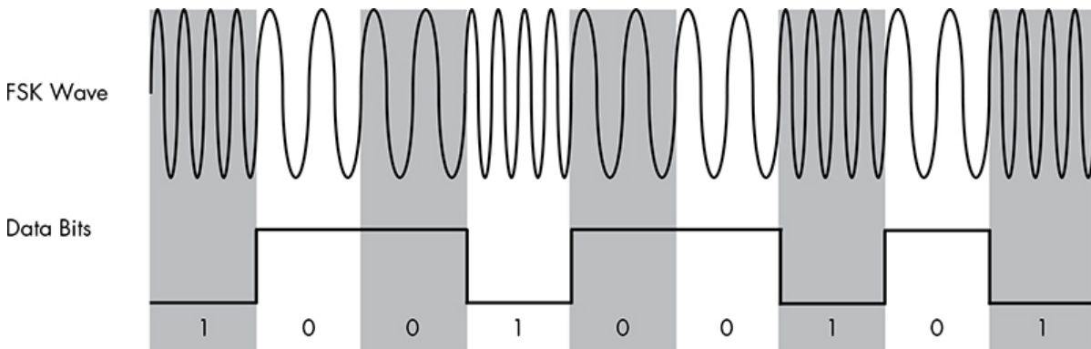
Figure 12-2: FSK modulation
