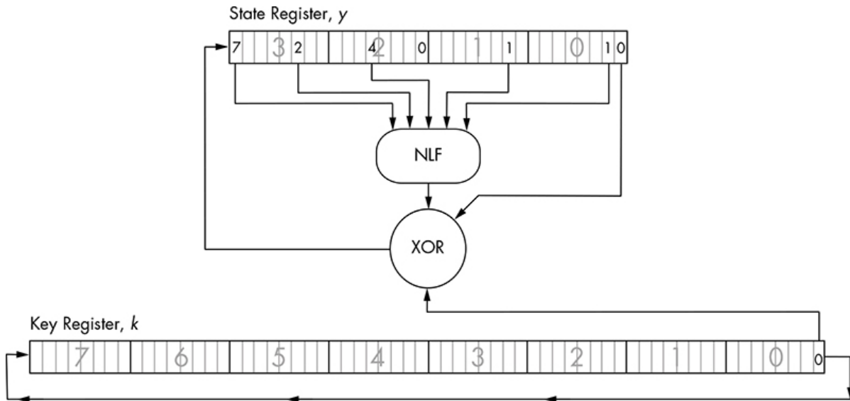
Figure 12-8: Keeloq algorithm
