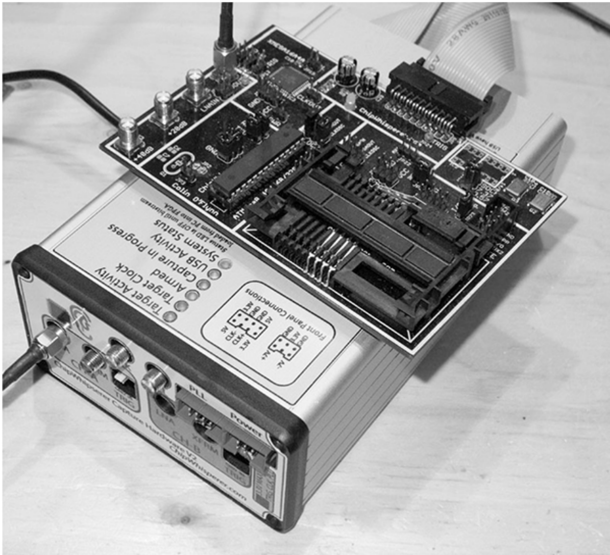
Figure 8-8: Wiring up the MultiTarget Victim Board
