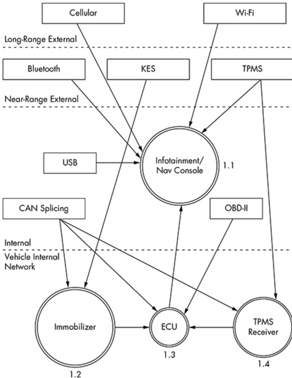
Figure 1-2: Level 1 map of inputs and vehicle connections
