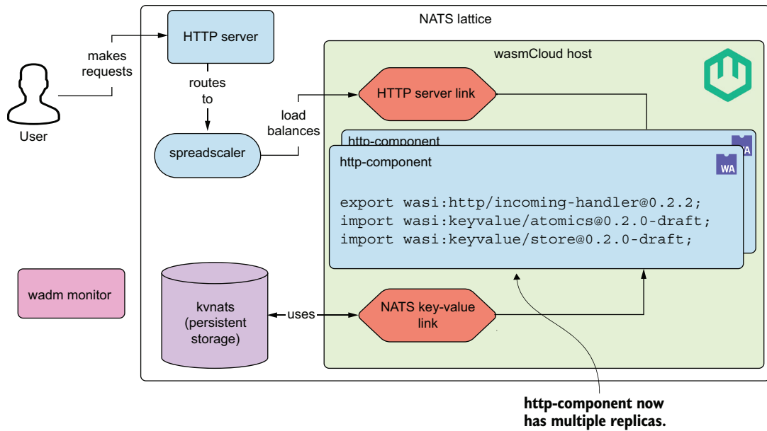
Figure 6.3 Updated architecture diagram for “Hello, World” wasmCloud app with 10 replicas of the http-component
