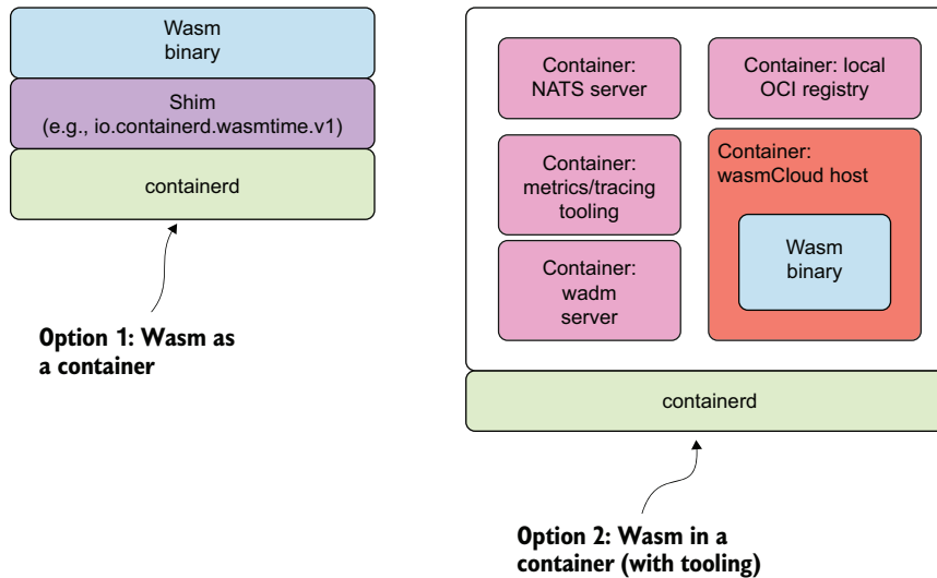
Figure 7.5 A comparison of two approaches to running Wasm in containers. On the left, Wasm runs directly inside a container using a lightweight shim. On the right, Wasm is packaged within a container alongside supporting infrastructure, as seen in wasmCloud’s approach, which includes components like the NATS server, a local OCI registry, and metrics/tracing tools.
