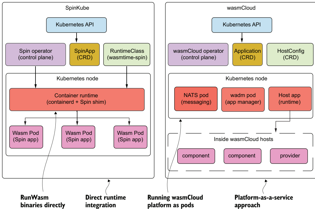
Figure 8.3 Architectural comparison of SpinKube and wasmCloud in Kubernetes. SpinKube (left) extends the container runtime with a Wasm shim to run Spin applications directly as pods. wasmCloud (right) deploys its platform components (NATS, wadm, and hosts) as regular Kubernetes pods, then orchestrates Wasm workloads within those hosts. Both approaches use CRDs and operators but integrate at different layers of the stack.
