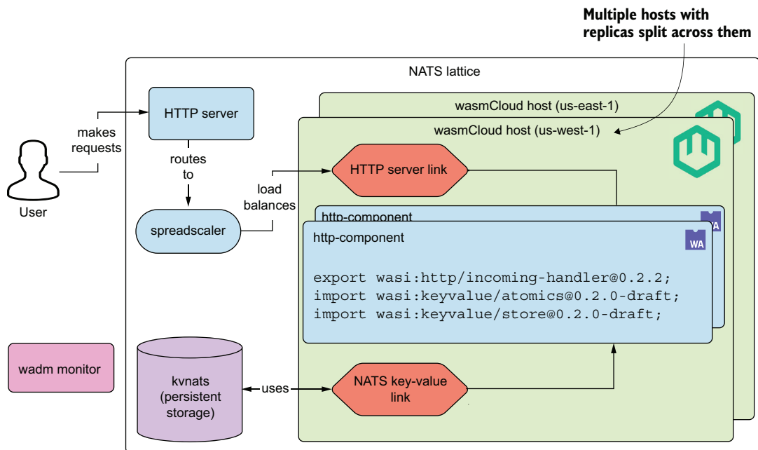
Figure 6.4 Updated architecture diagram for “Hello, World” wasmCloud app with 10 replicas of the http-component split across different hosts and regions (i.e., us-east-1 and us-west-1)
