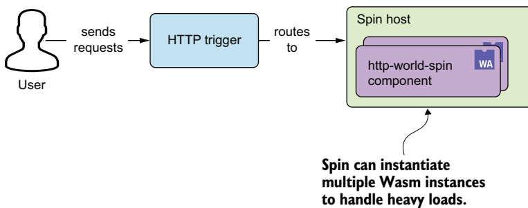
Figure 6.5 Spin's event-driven setup for Wasm microservices
