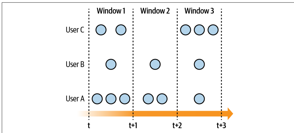
Figure 9-10. Tumbling windows
