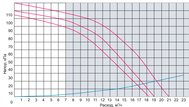
OD-90.0-80-120-P3-WL
