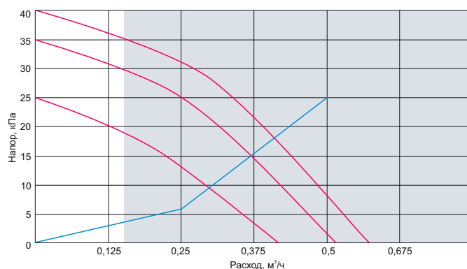
OD-2.5-20-40-P1-WL
