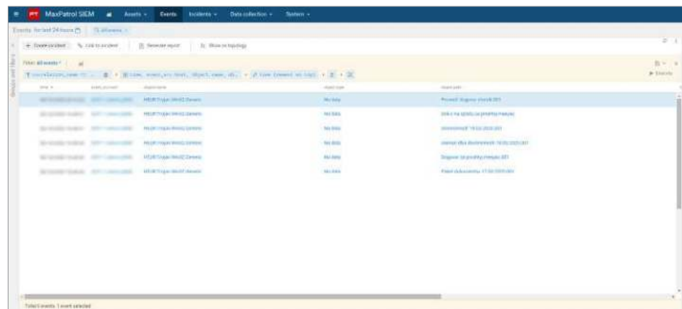
Figure 9. Detection of phishing with MaxPatrol SIEM
