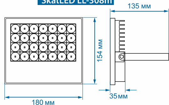
SkatLED LL-308m
