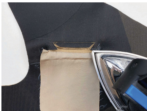
16. Turn the welt with its lining to the wrong side of the front piece and smooth it out. Press the welt with its lining.
