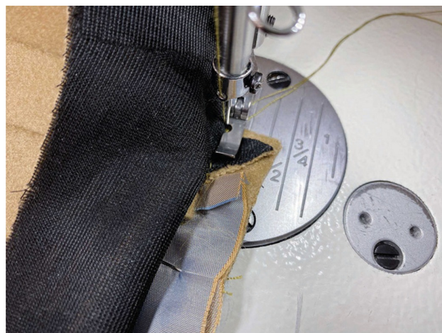
19. Machine-stitch the pocket side corners to the chest pocket welt piece, going back and forth three times.
